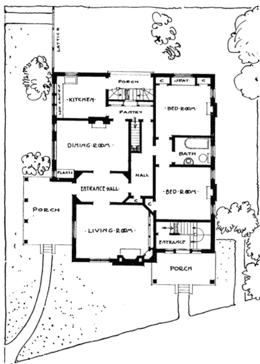
PLOT OF LOT AND FIRST FLOOR.
