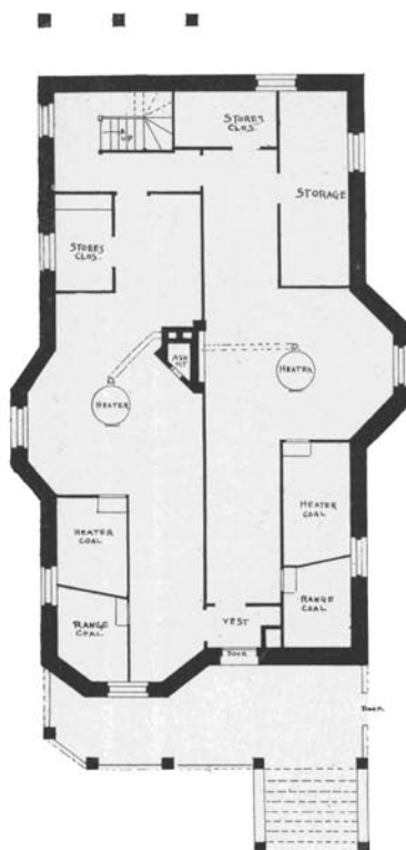
CELLAR PLAN
