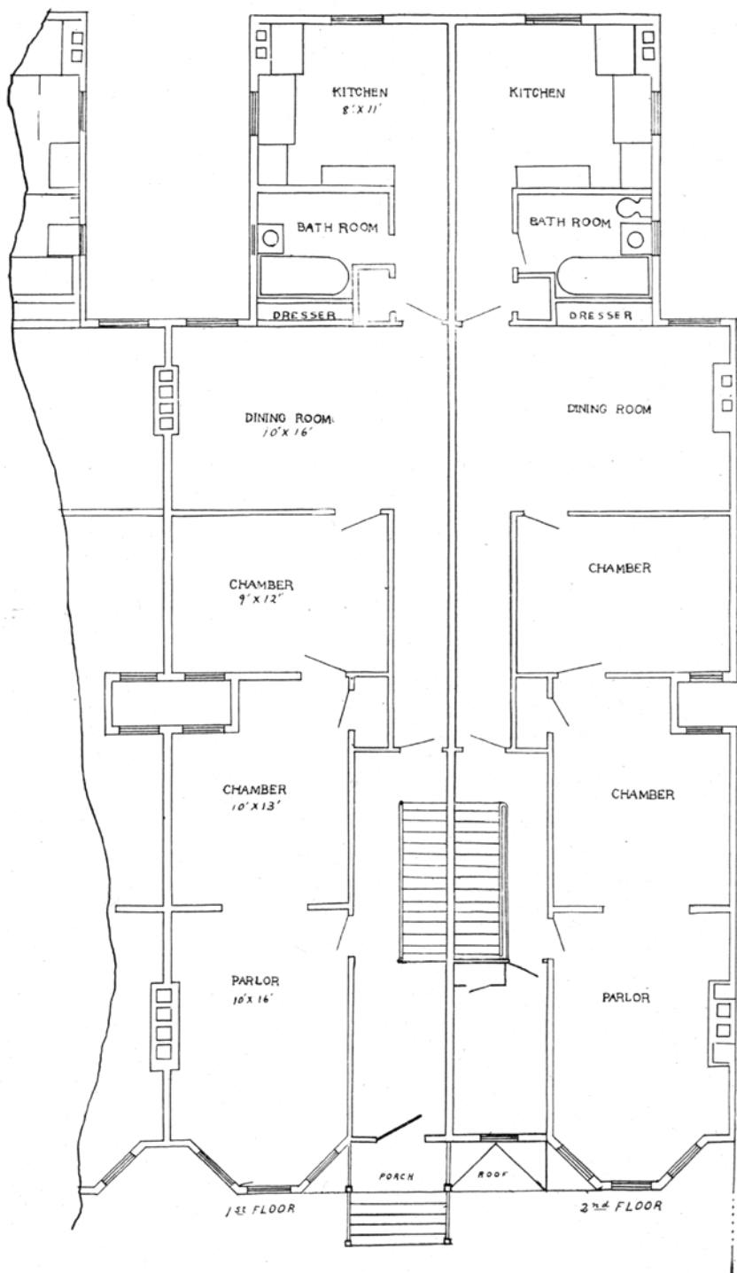
GROUP OF THREE TWO FAMILY HOUSES ON DECATUR AVENUE, BEDFORD PARK, N. Y.
