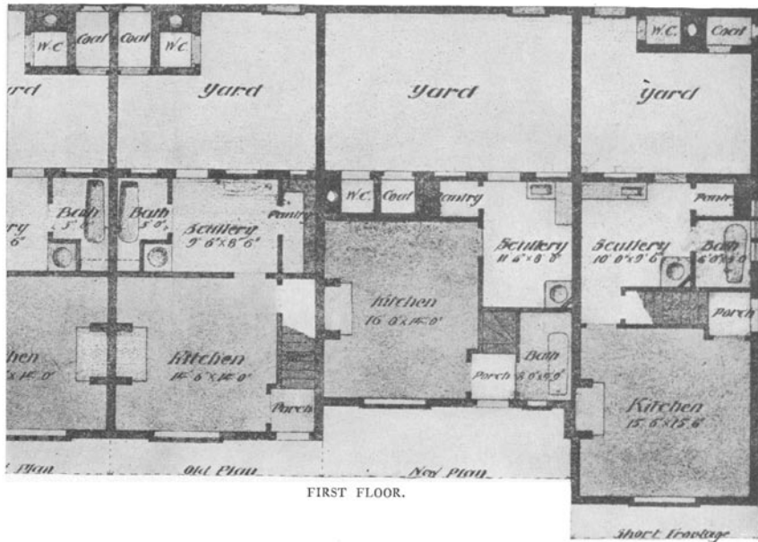
BLOCK OF SEVEN COTTAGES, PORT SUNLIGHT, ENG.
