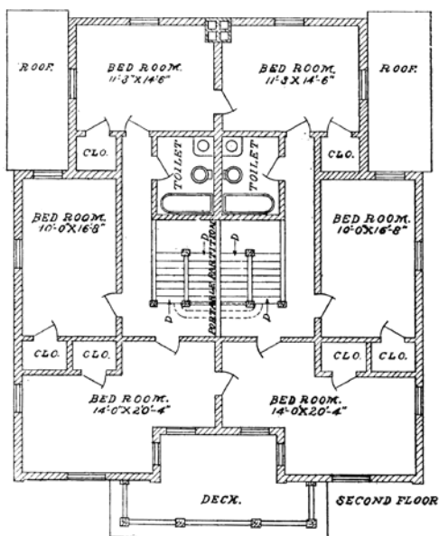
TWO FAMILY HOUSE, EL PASO, TEX.
