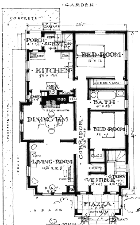
A $3800 TWO FAMILY HOUSE, BOSTON, MASS.
