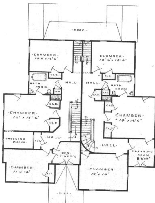
SECOND-FLOOR PLAN -
