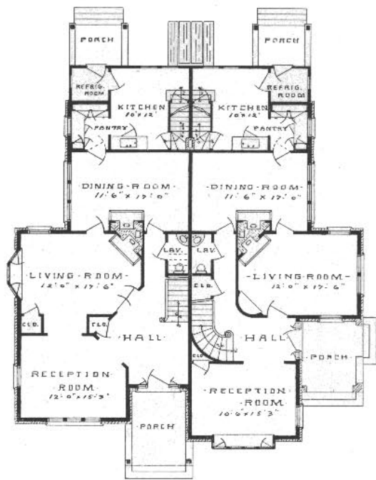
FIRST-FLOOR PLAN -
