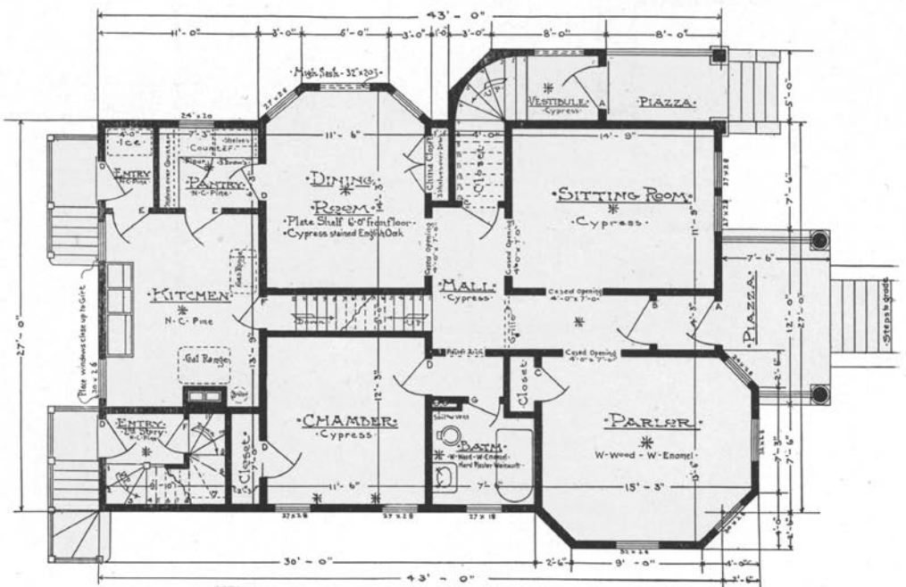
FIRST FLOOR.
