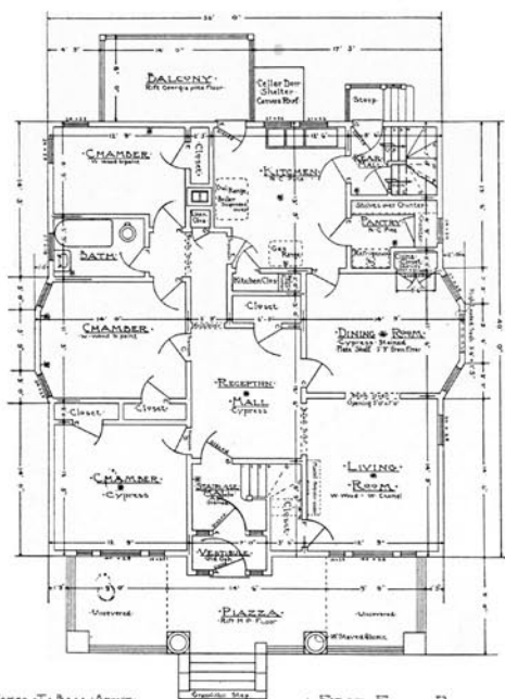
THREE FAMILY HOUSE, DORCHESTER, MASS.
