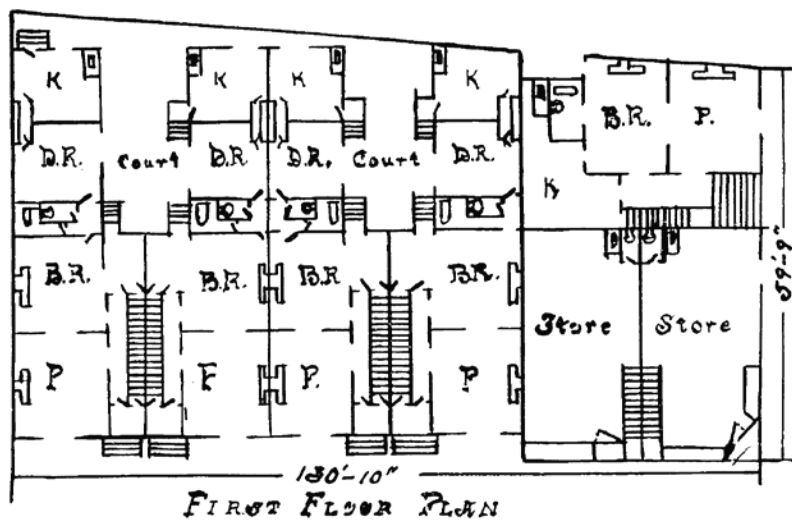
TAYLOR APARTMENTS, ST. LOUIS, MO.
