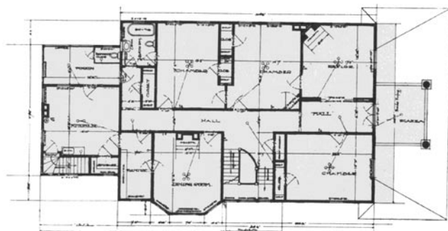
TWO FAMILY HOUSE, JACKSONVILLE, FLA. McClure & Holmes, Architects.
