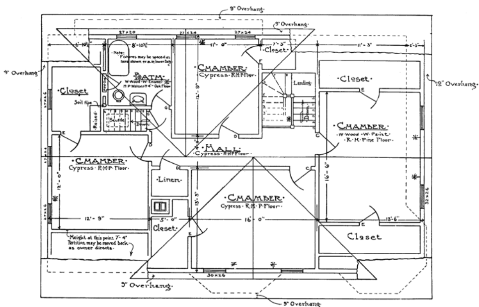
THIRD FLOOR.
