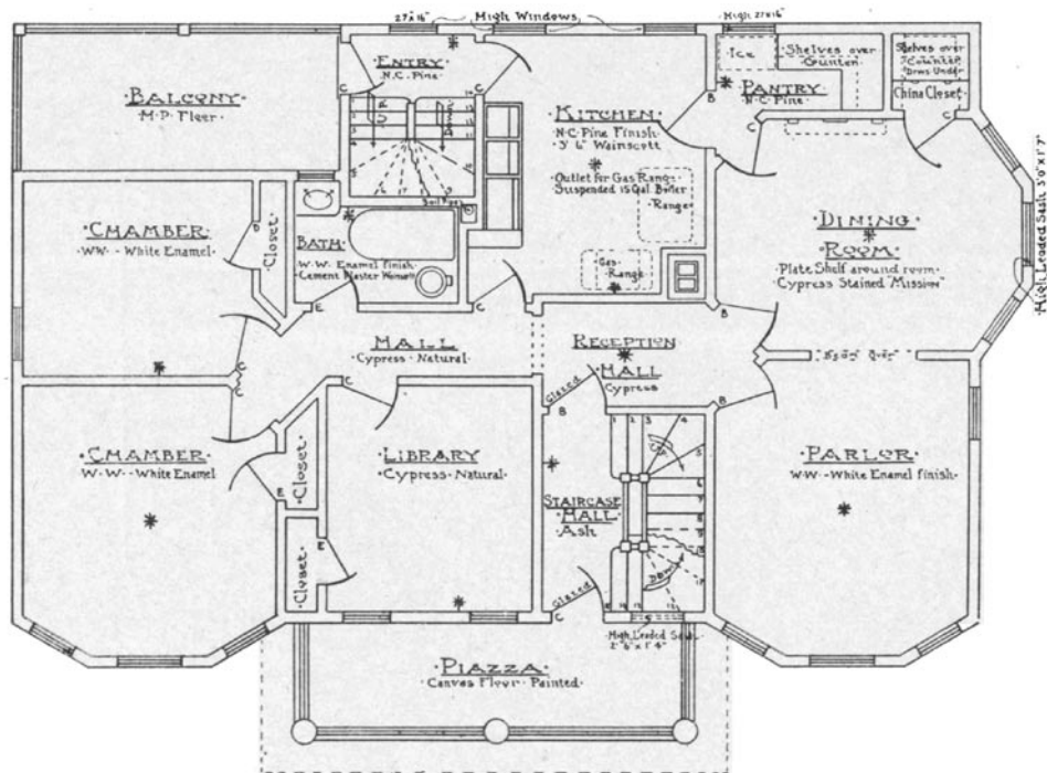
THREE FAMILY HOUSE.
