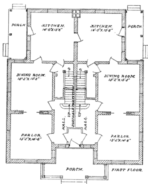
TWO FAMILY HOUSE, EL PASO, TEX.
