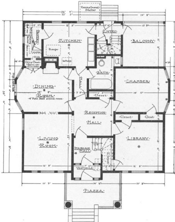
THREE FAMILY HOUSE.
