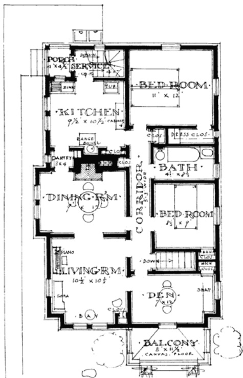
A $3800 TWO FAMILY HOUSE, BOSTON, MASS.
