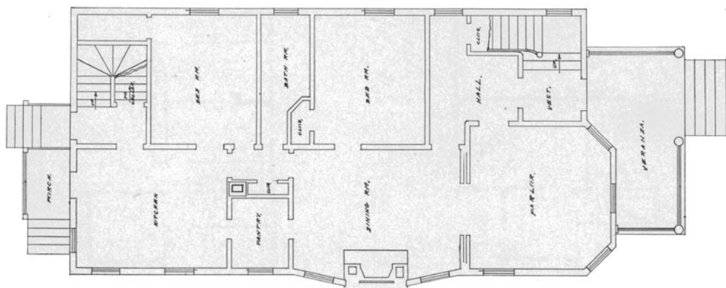
THREE FAMILY HOUSE, WATERBURY, CONN.
