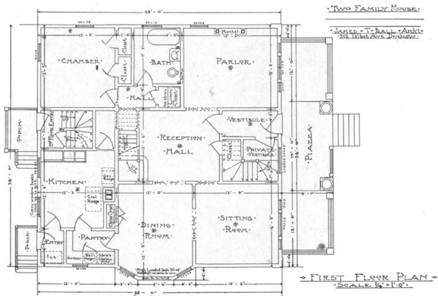
TWO FAMILY HOUSE.
