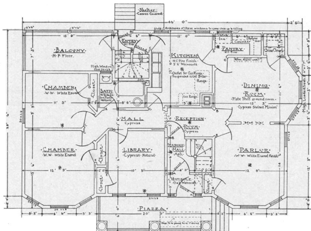
FIRST FLOOR.
