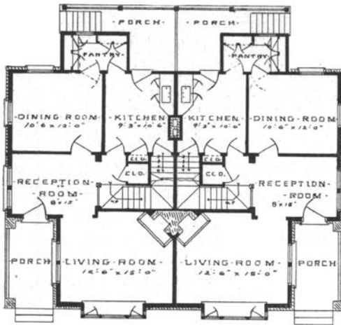
- FIRST-FLOOR PLAN -
