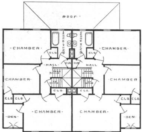
- SECOND-FLOOR PLAN -
