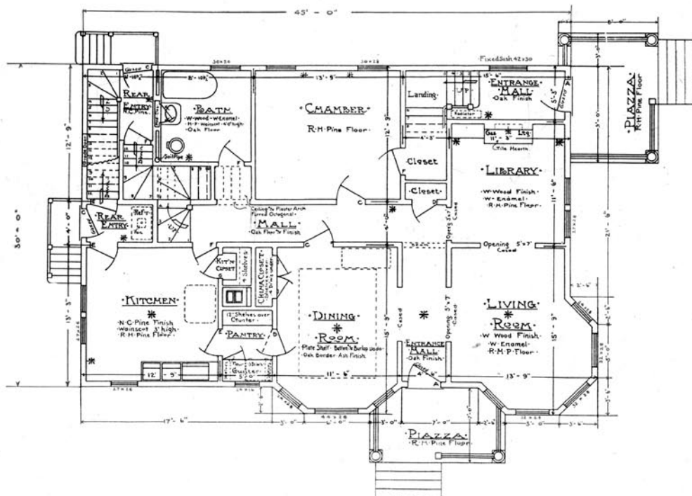
FIRST FLOOR. TWO FAMILY HOUSE.
