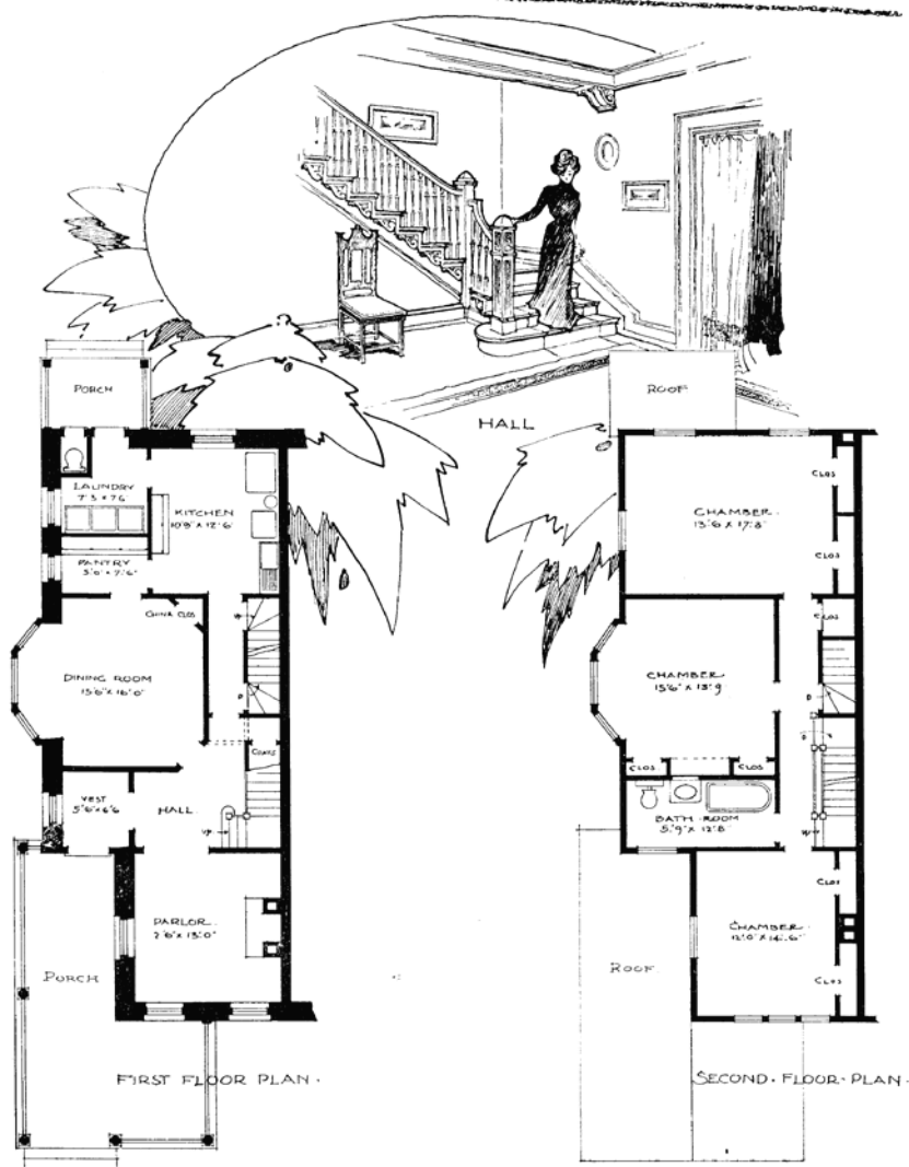
TWO FAMILY HOUSE.
