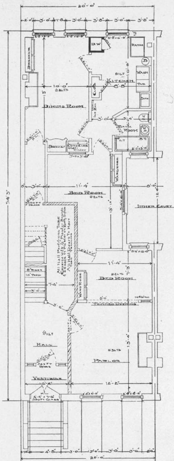
FIRST FLOOR.
